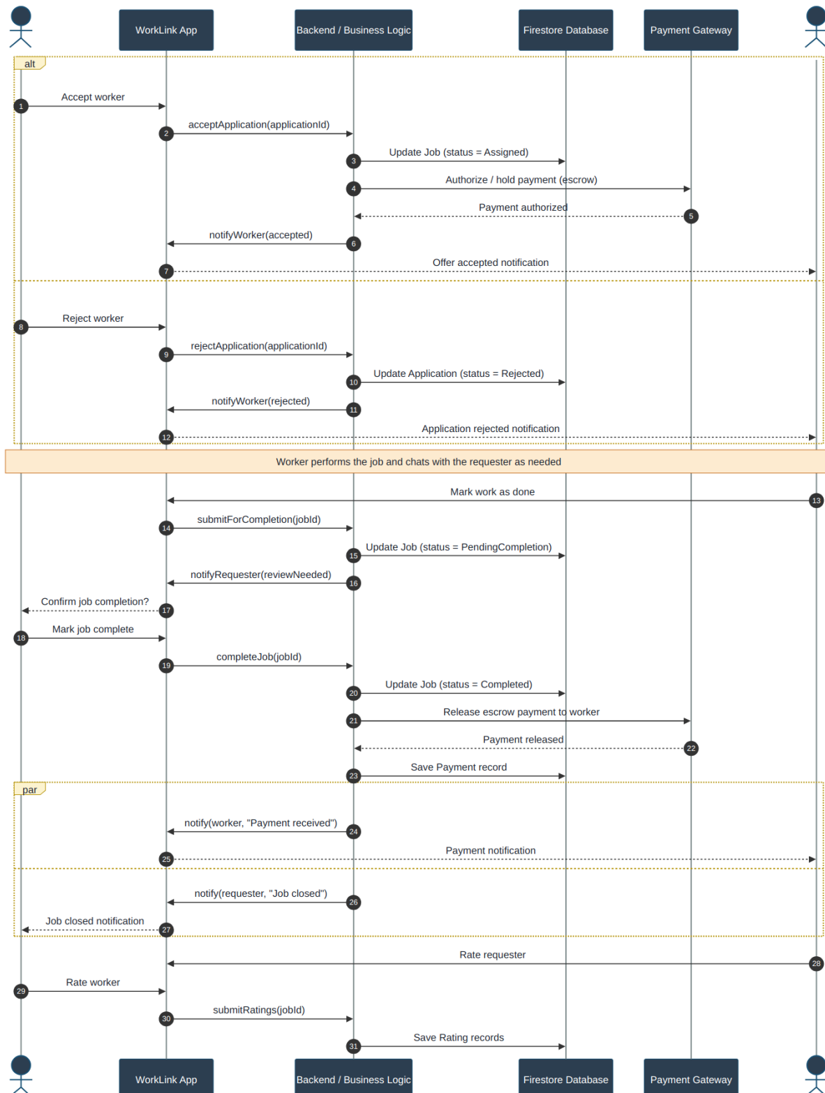
Figure 3b — Hiring, execution, payment, and rating sequence
